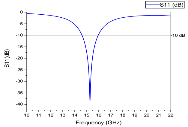
a. Return Loss Vs Frequency
