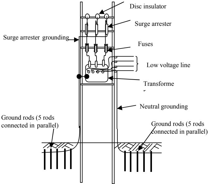
Figure-1: Grounding of Pole Mounted Transformer
