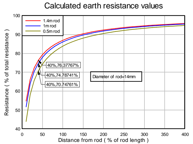
Fig-1: Variation of ground resistance with distance from ground electrodes
